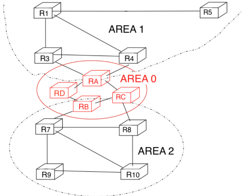
Figure 5.50: OSPF areas
